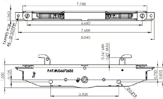
1148-D5 2-HOOK Mortise lock
